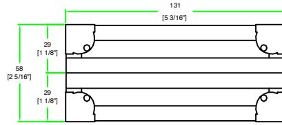
LEFT VIEW
