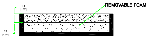
C-C VIEW
