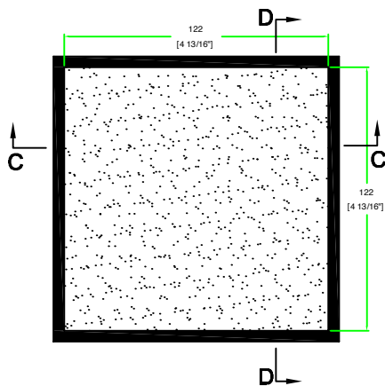
TOP VIEW OF BASE
