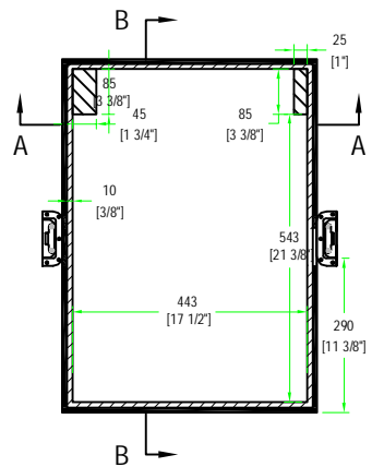
TOP VIEW OF BASE
