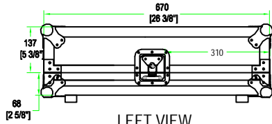
LEFT VIEW
