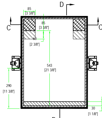
TOP VIEW OF COVER
