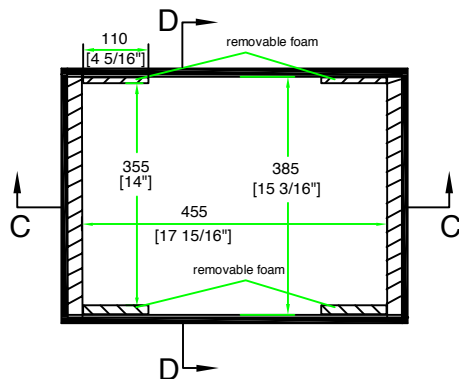
TOP VIEW OF BASE
