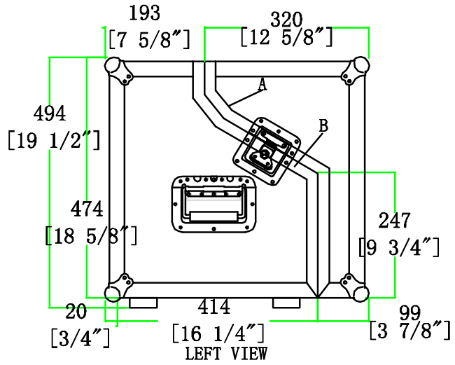
LEFT VIEW
