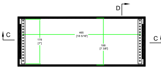
TOP VIEW OF BASE
