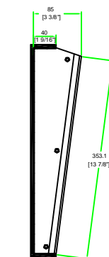
D-D VIEW
