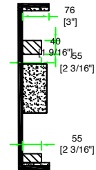
B-B VIEW
