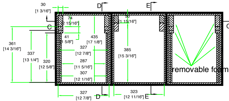
TOP VIEW OF BASE
