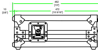
LEFT VIEW
