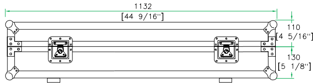
BACK VIEW
