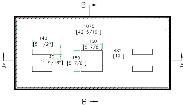
TOP VIEW OF COVER
