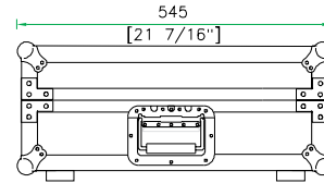
LEFT VIEW
