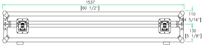
BACK VIEW
