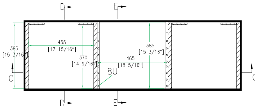
TOP VIEW OF BASE
