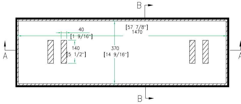
TOP VIEW OF COVER
