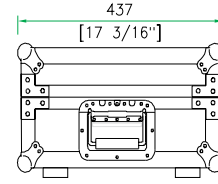
RIGHT VIEW
