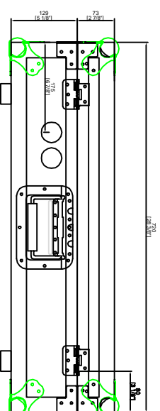
BACK VIEW
