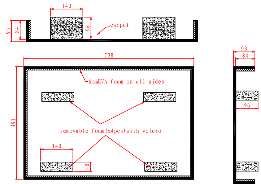
TOP VIEW OF BASE
