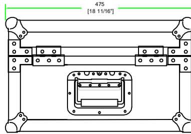
LEFT VIEW
