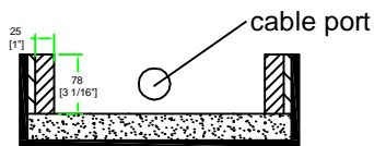
C-C VIEW
