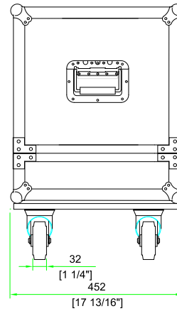
LEFT VIEW
