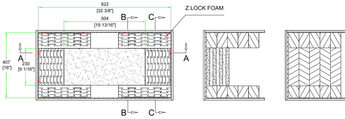
B-B VIEW
