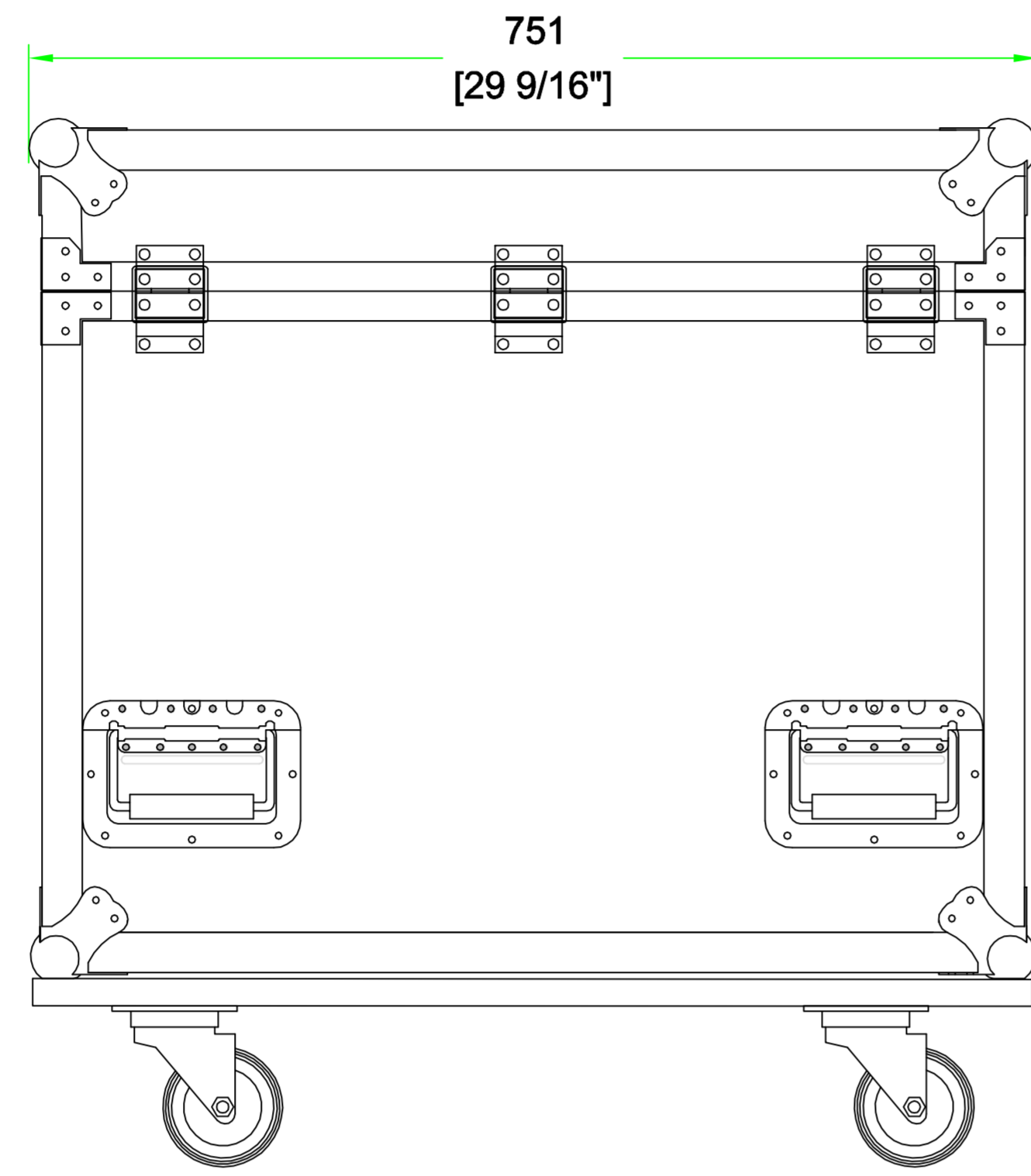
BACK VIEW
