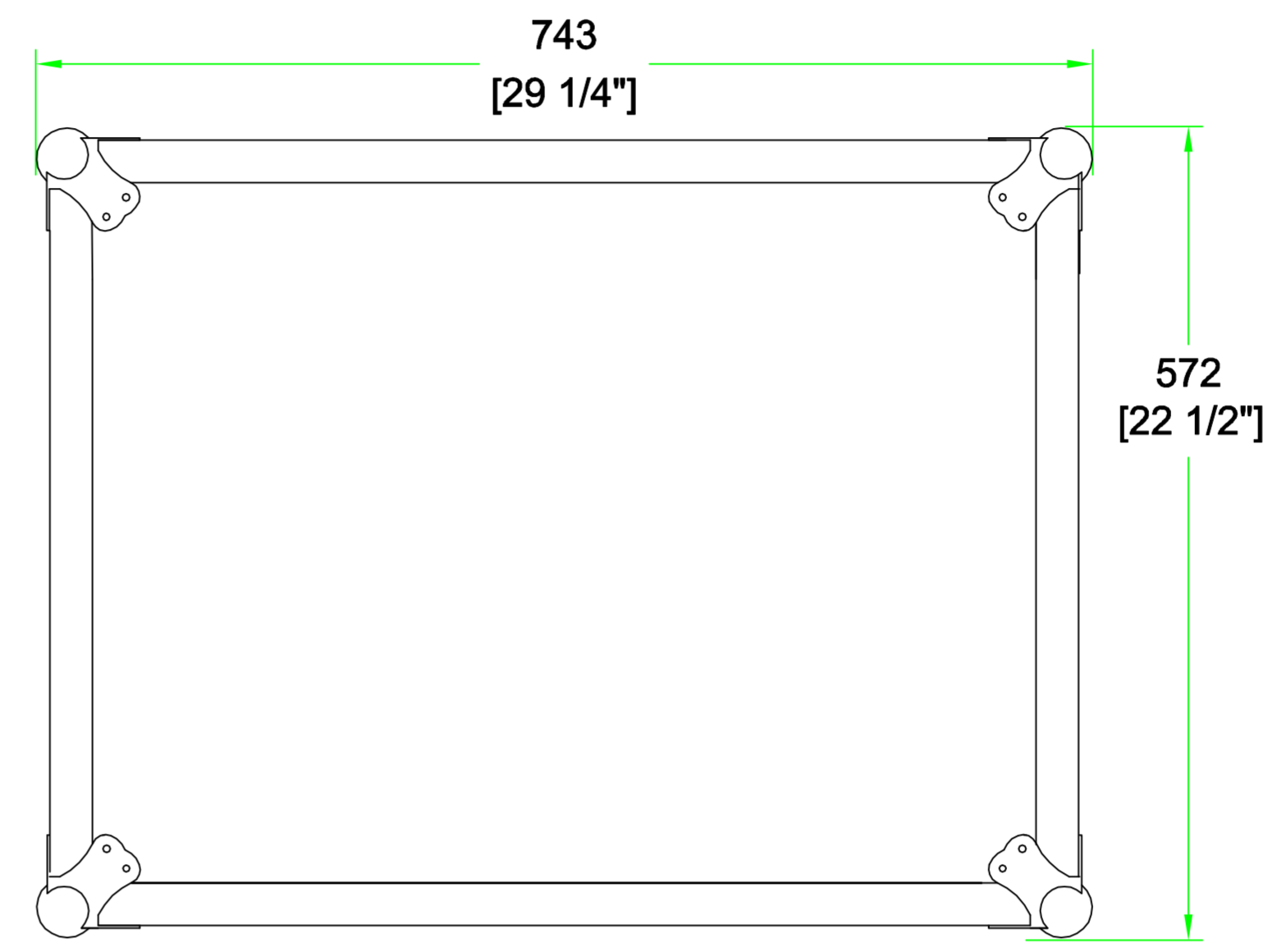
TOP VIEW
