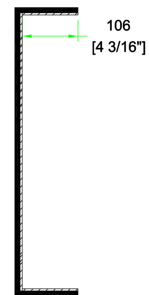
B-B VIEW
