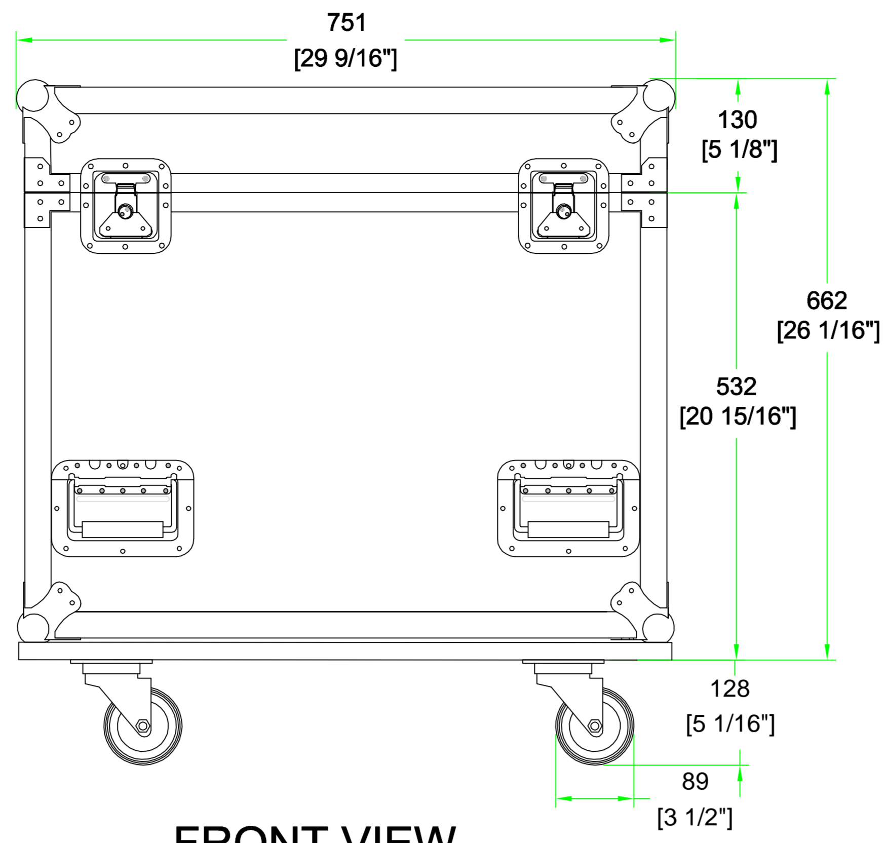
FRONT VIEW
