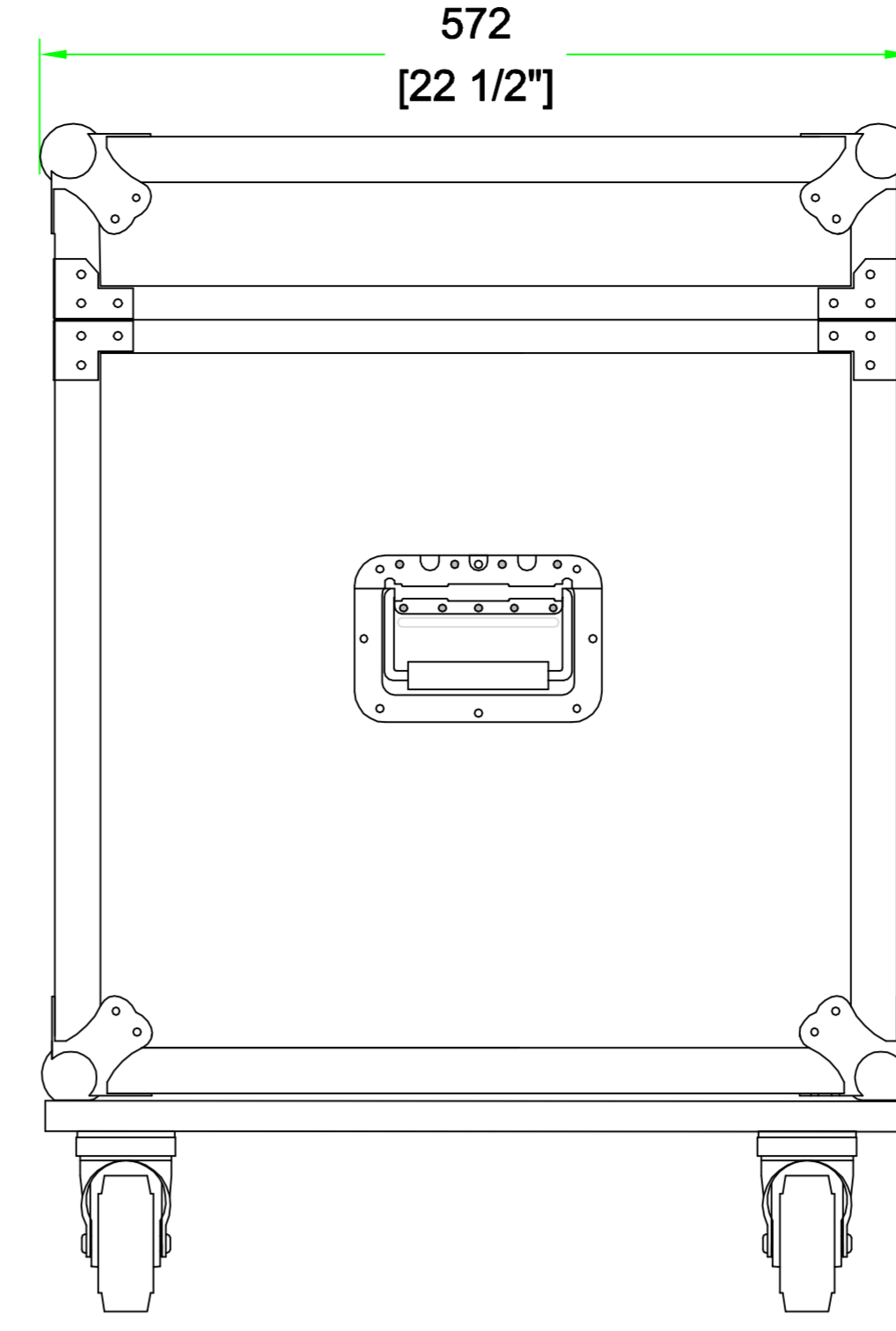
LEFT VIEW
