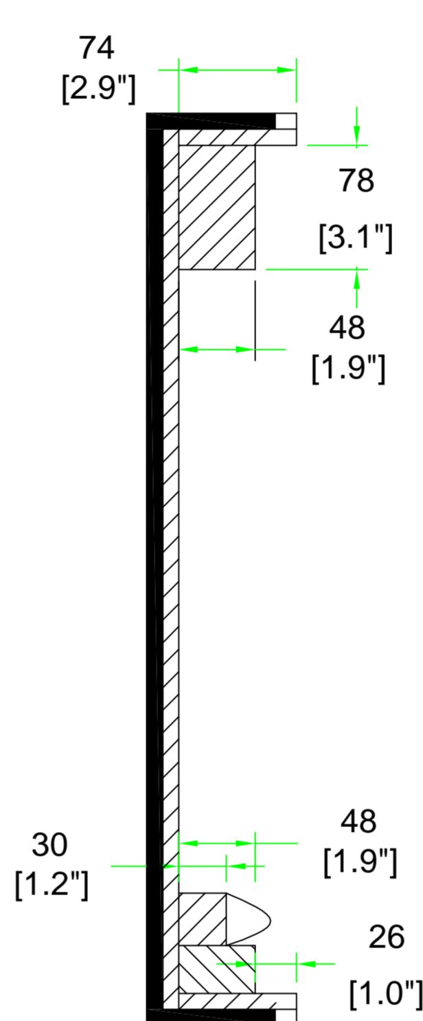
D-D VIEW
