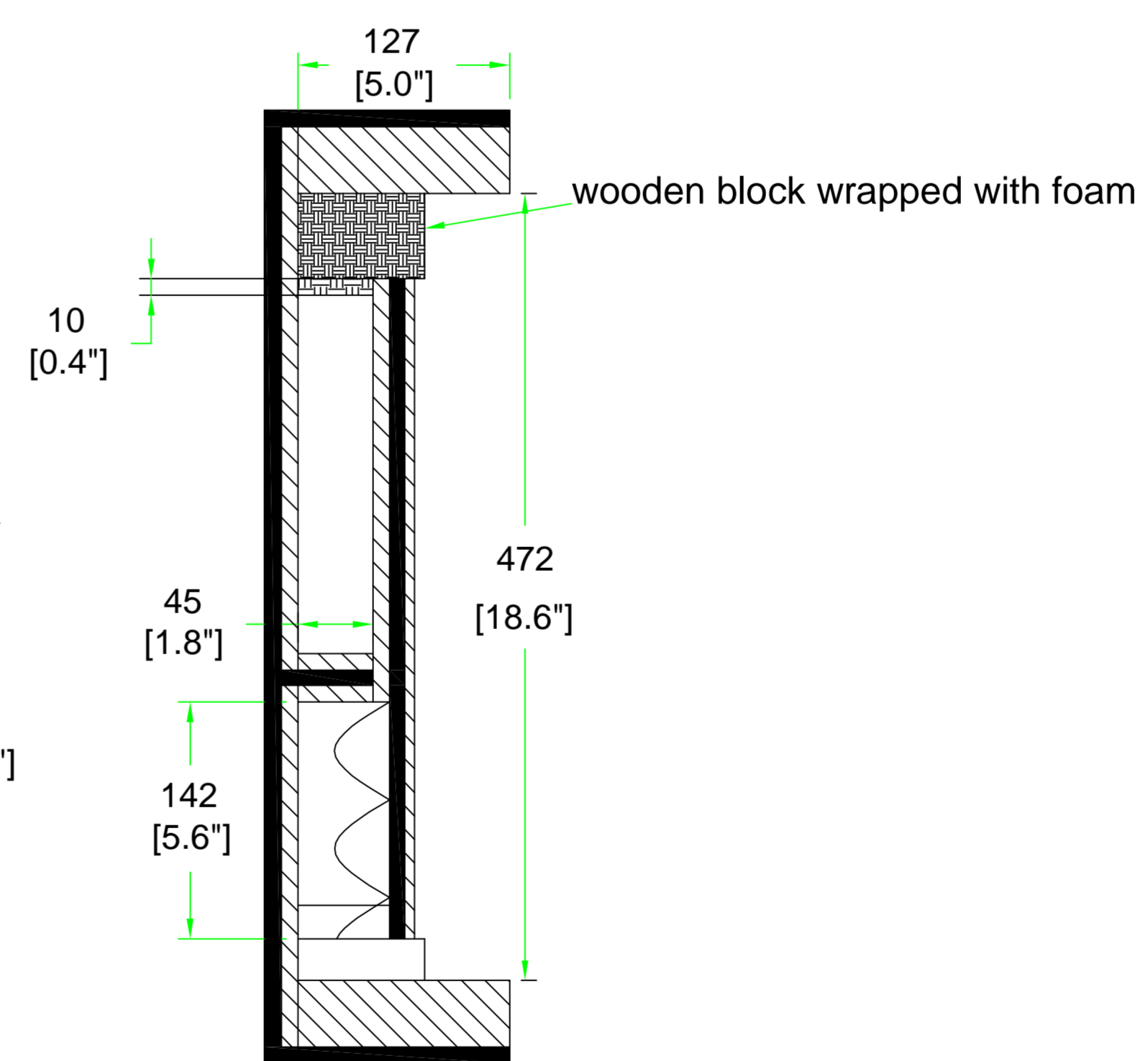
B-B VIEW
