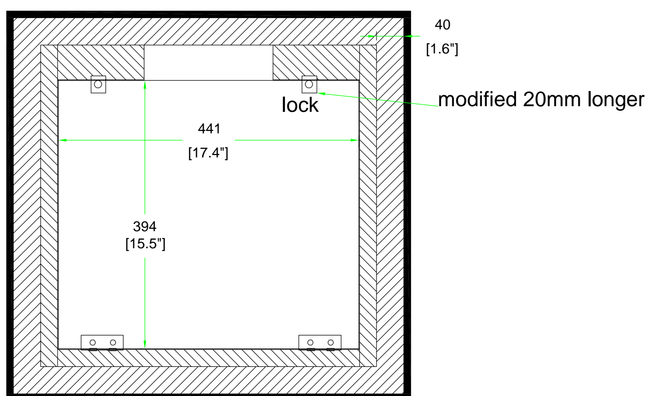
TOP VIEW OF COVER
