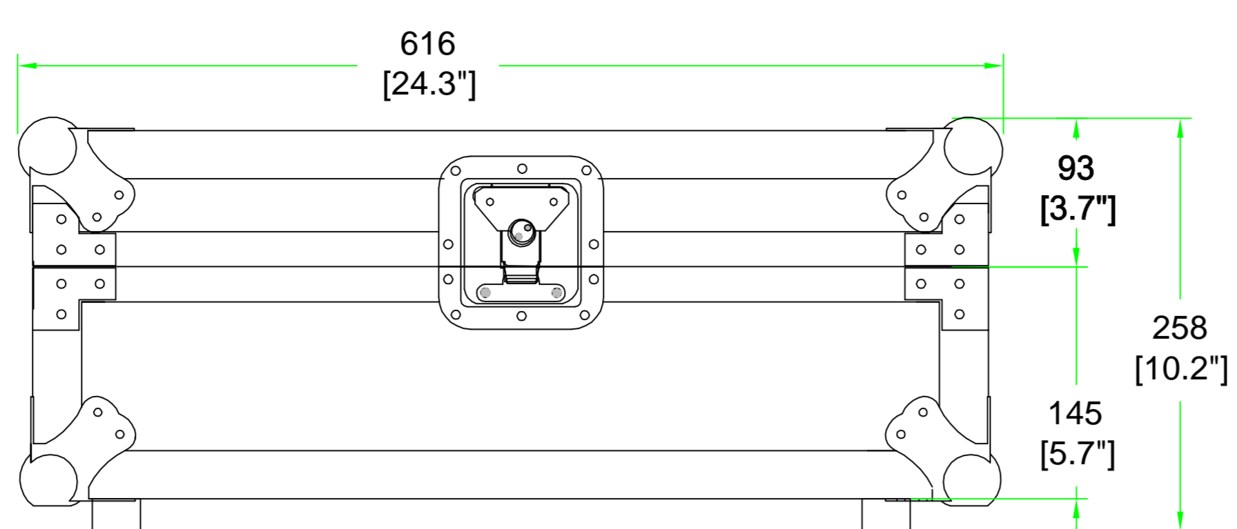
FRONT VIEW
