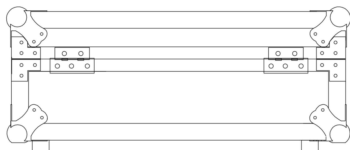
BACK VIEW
