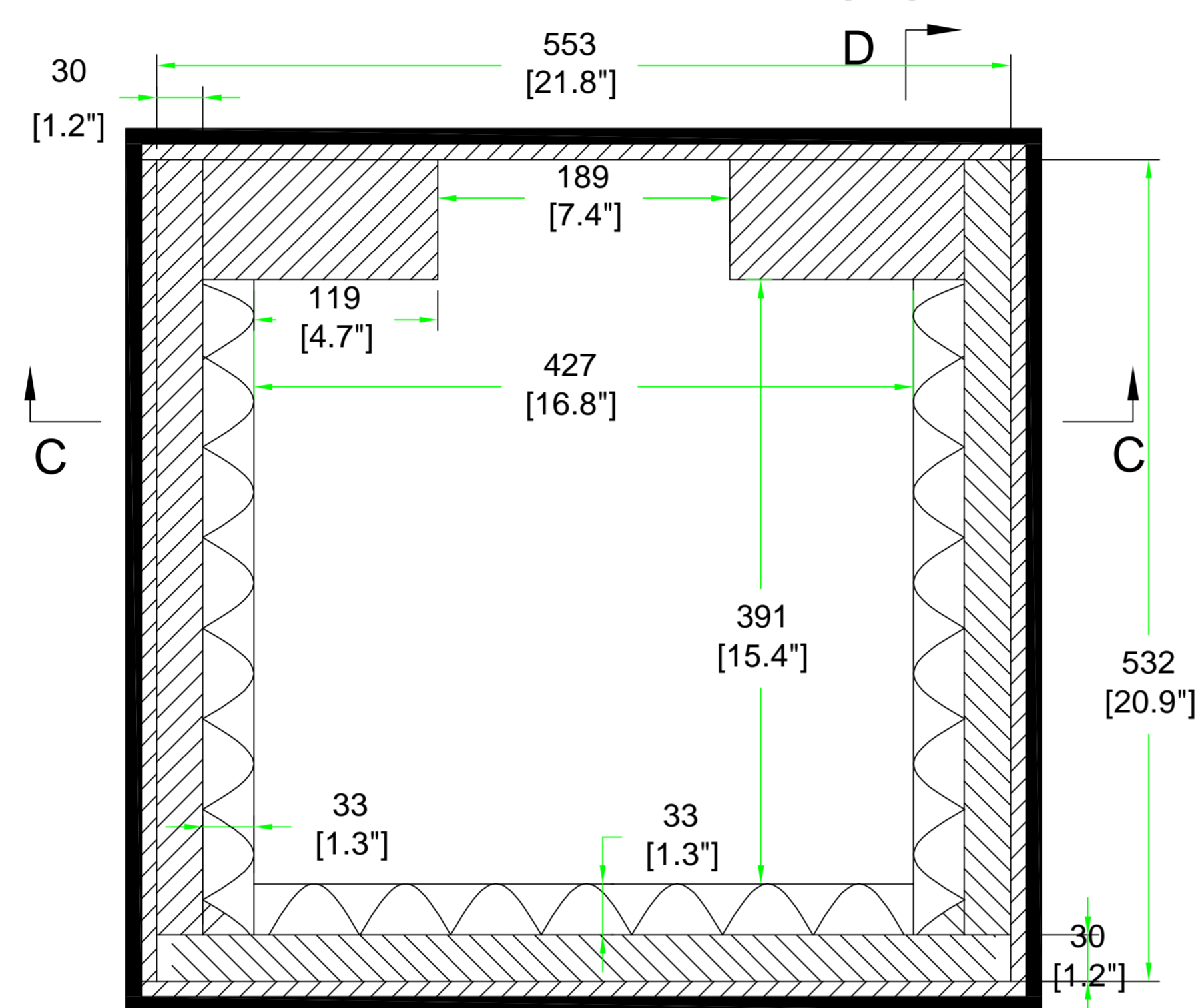
TOP VIEW OF BASE
