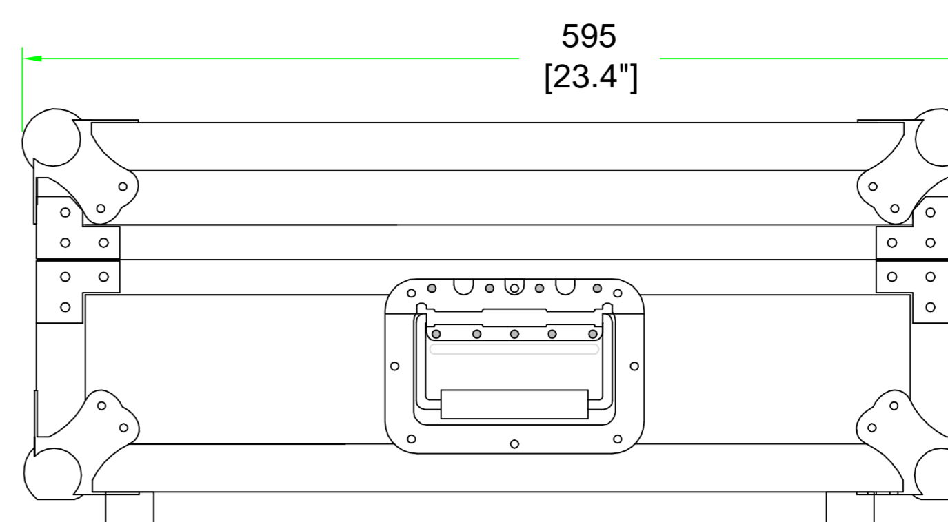
RIGHT VIEW
