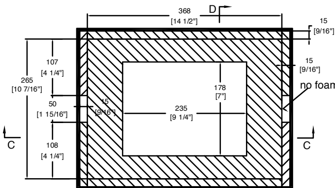
TOP VIEW OF BASE
