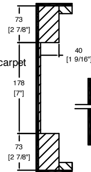
D-D VIEW
