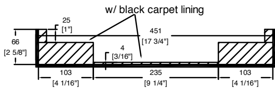
C-C VIEW
