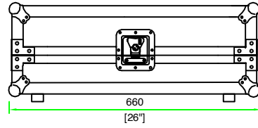
LEFT VIEW
