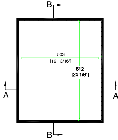
TOP VIEW OF COVER
