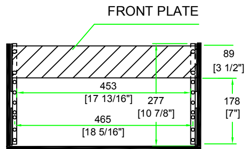
INSIDE VIEW
