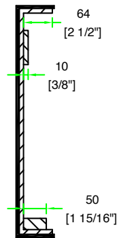
B-B VIEW
