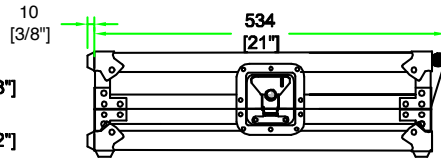
LEFT VIEW
