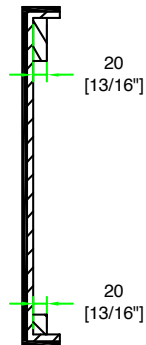
D-D VIEW
