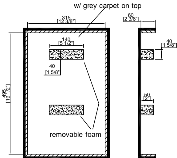
TOP VIEW OF COVER
