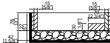
C-C VIEW
