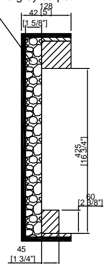
D-D VIEW
