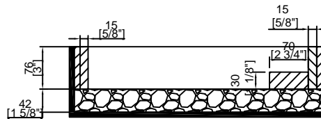
C-C VIEW
