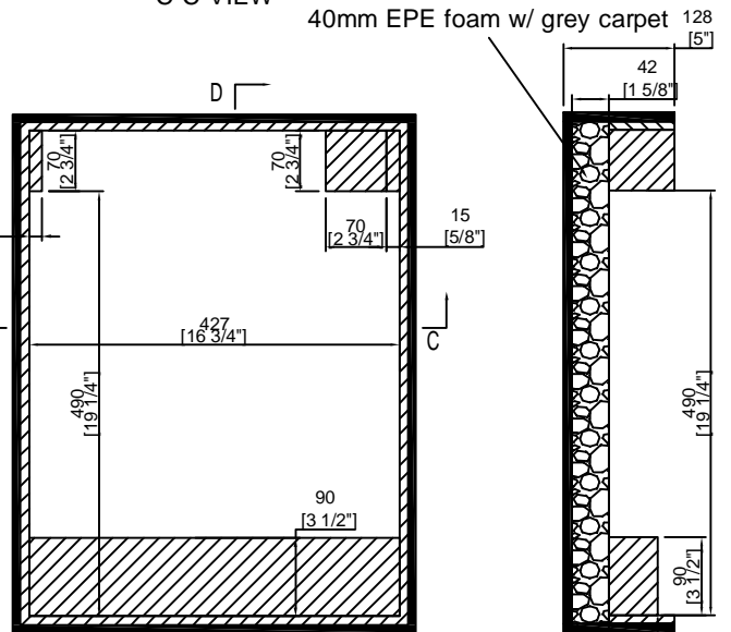
C-C VIEW
