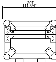
LEFT VIEW
