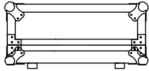
BACK VIEW
