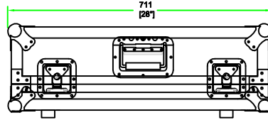
LEFT VIEW
