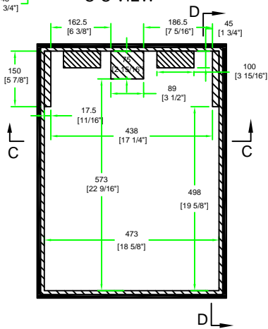
C-C VIEW
