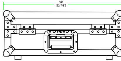
LEFT VIEW
