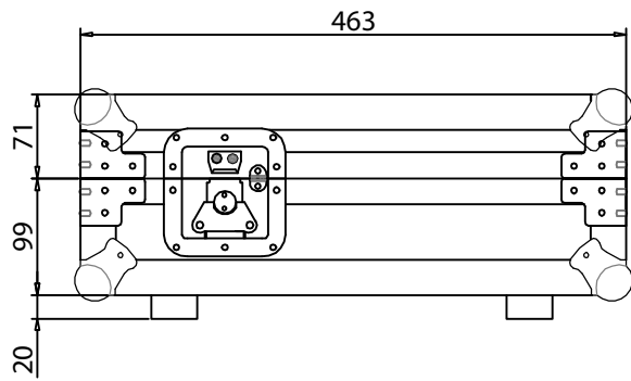
RIGHT VIEW
