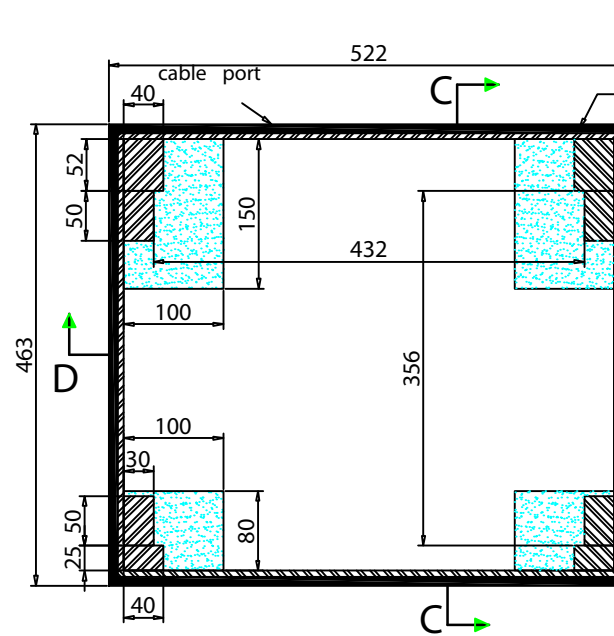
TOP VIEW OF COVER
