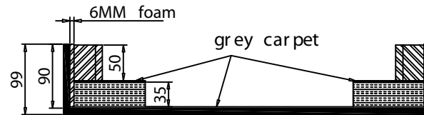
D-D VIEW
