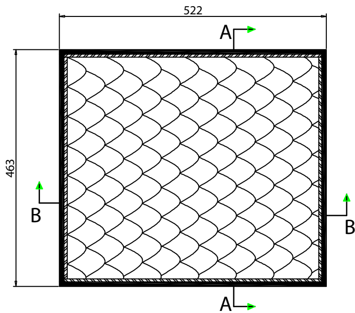
TOP VIEW OF BASE
